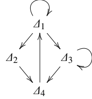
Fig. 4: A network of unwinding components
